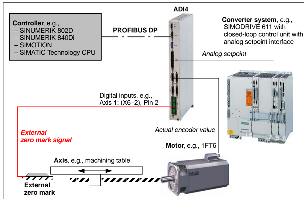
Fig. 3-6 Basic system structure: Homing using external zero mark
