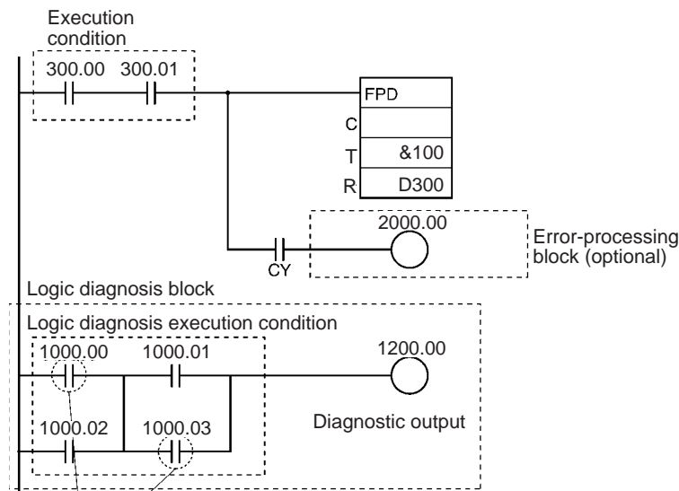
The diagnostic output (CIO 200.00) remains OFF because these input conditions are OFF.
