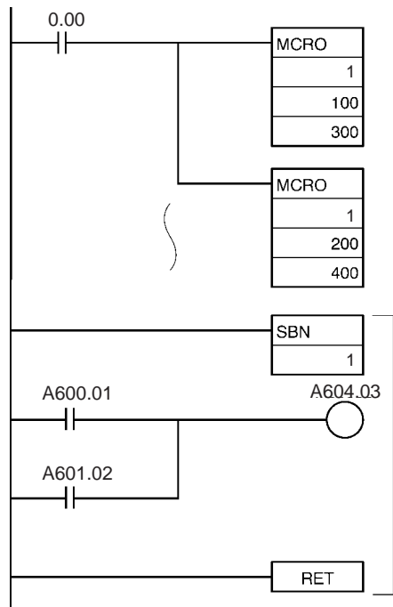
Subroutine 1
