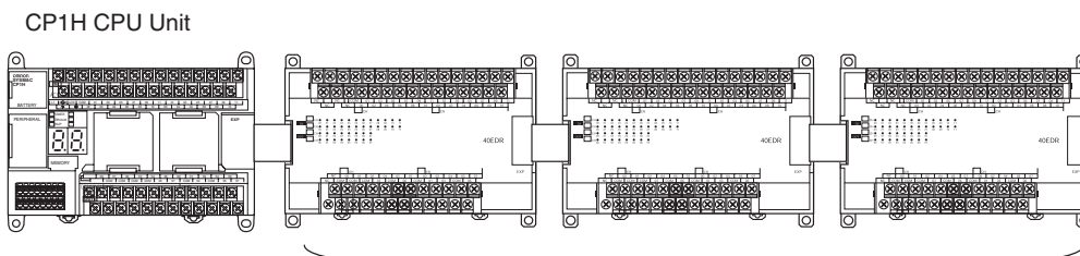
A maximum of 7 CPM1A-series Expansion I/O Units or Expansion Units can be added.
